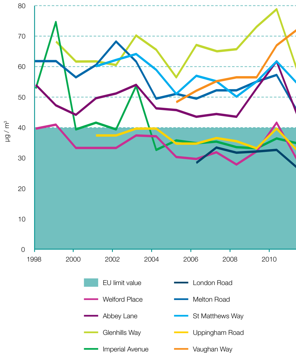
Exhibit 3: Mean annual NO 2 concentrations across Leicester
